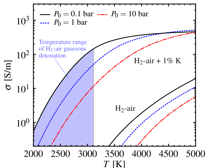
Figure 37: The equilibrium electrical conductivity is shown as a function of pressure and temperature for a stoichiometric H 2 -air mixture. Seeding by potassium drastically increases the electrical conductivity.
