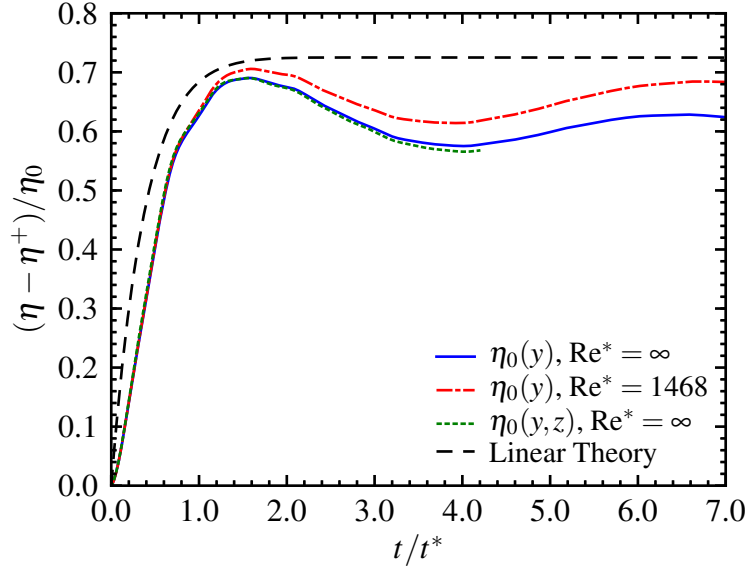
Figure 53: Time evolution of the mixing layer width for the single-mode RMI in a magnetized plasma with \beta = 10 and initial conditions of M_s = 1.5 , k_0\eta_0 = 0.1 , A = 0.5 . The results for two- and three-dimensional numerical simulations using both the ideal ( Re^* = \infty ) and resistive MHD equations are compared to the linear theory, where Re^* = Re_m^* are both computed from the reference parameters.
