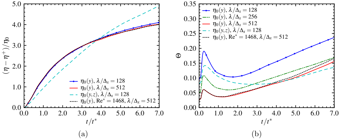
Figure 34: Time history of (a) the normalized mixing length and (b) the mixing fraction in single-mode RMI at the different grid resolutions ( \Delta x_1, \Delta x_2 ) and for inviscid and viscous simulations.
